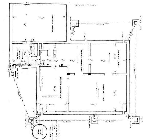
FUNDERING.
